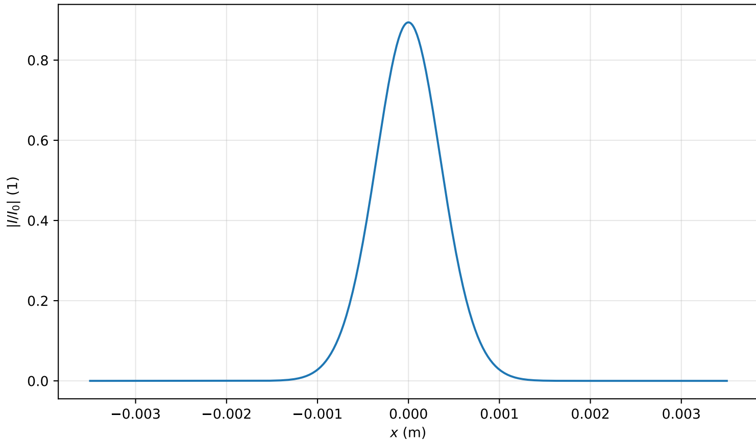
Intensity profile I(x, y = 0, z = 0.955m)/I_0 , P_{in}=0.2P_{cr} , artificial time
